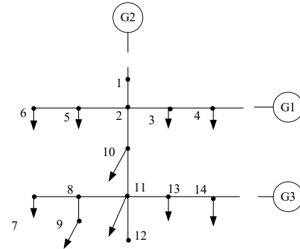
Figure 5-1 Improved IEEE13-bus system diagram
