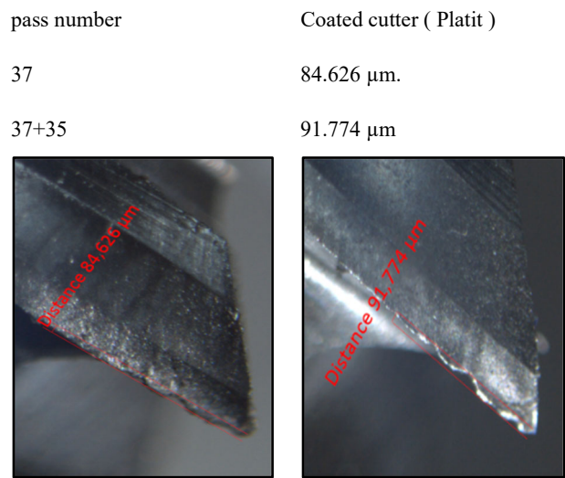
Fig. 5. Wear is visible on the tool after machining.
