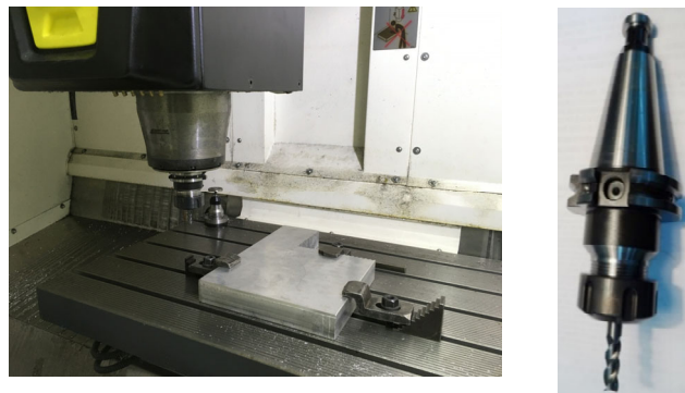
Fig. 6. Machined by milling machine.
