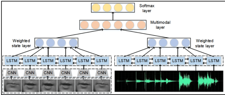
Fig. 5. Structure of the RNN multimodal model.
