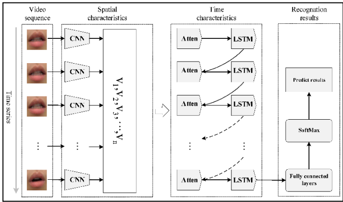
Fig. 4. Example of a convolutional neural network architecture for lip motion analysis.
