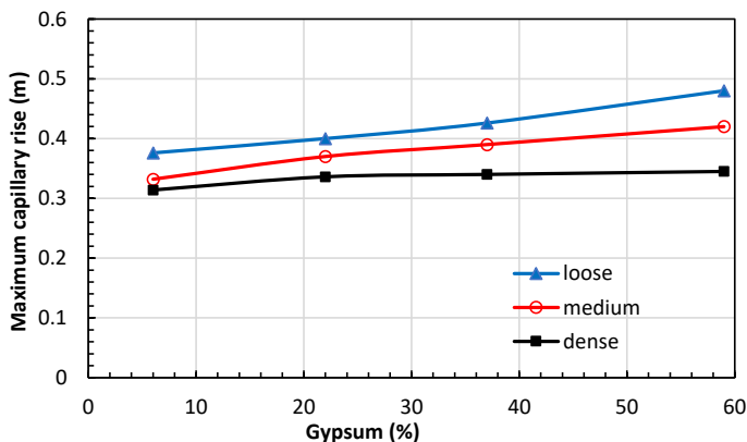
Figure 9: The relationship between gypsum percentage and maximum capillary rises for different soil states.
