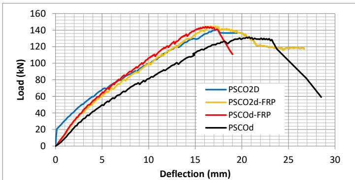
Figure 14: Effect of opening location and strengthening due to circular openings.
