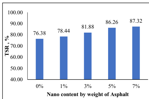
Figure 15: TSR value of neat and nano-modified asphalt.
