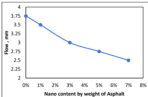
Figure 11: Flow value of Marshall test with different nano content.
