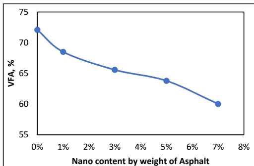
Figure 13: Voids filled with asphalt value of Marshall test with different nano content.
