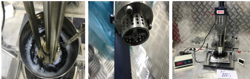
Figure 4: Mixing neat asphalt with nanomaterial using HSMd.
