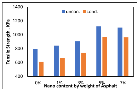
Figure 14: The tensile strength value of neat and nano-modified asphalt.
