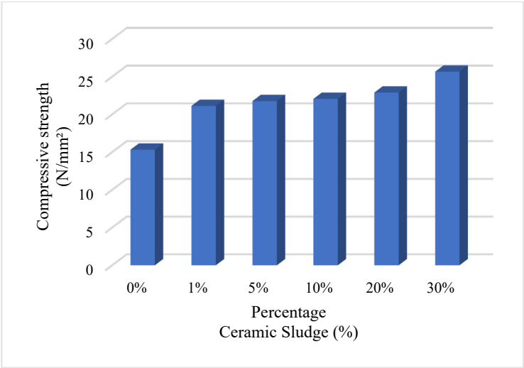
Fig. 2. Compressive strength between different percentage of sludge.
