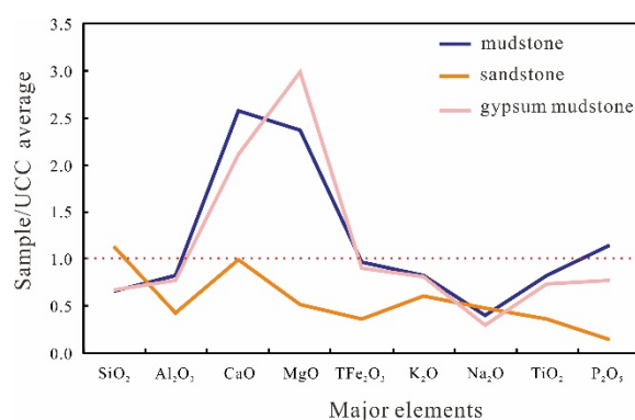
Fig. 4 The mean value line chart of major elements / UCC of different lithology in E3l of H6 well
