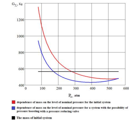
Fig. 4. Comparative dependency graph of systems with relief valve at k_f = 2 .
