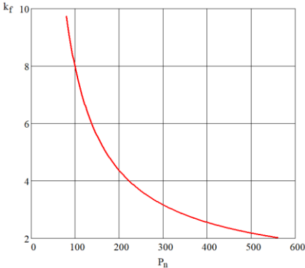
Fig. 3. Graphical dependence of coefficient k_f for drives using the example of AMHT drive.
