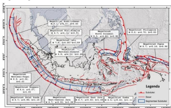
Fig. 2 Indonesia's Segmentation Map and Subduction Mmax
