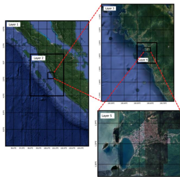
Fig. 6 Form of Multilayer Area Simulation in the COMCOT Program
