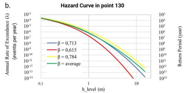
Fig. 12 Comparison of Hazard Curves based on: a. Value a and Value b, b. Logic Tree ( \beta )
