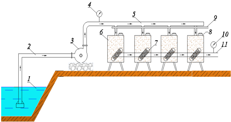
Fig. 1. Filtration system
