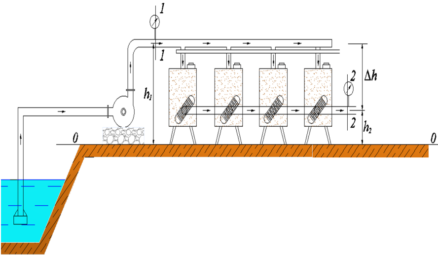
Fig. 2. Calculation scheme
