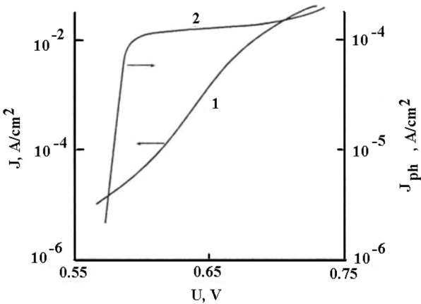
Fig. 2. Dependence of dark current density J(1) , and photocurrent J_{ph}(2) on voltage. T=55 K, \lambda=10.6 \mu m
