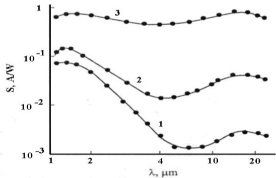
Fig. 1. Spectral sensitivity of injection photodiode. Bias voltages U , V: 1- 1, 2-10, 3-20, T=55 K.
