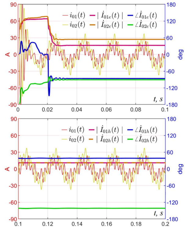
Fig. 4. Comparison of equivalent synchrophasors
