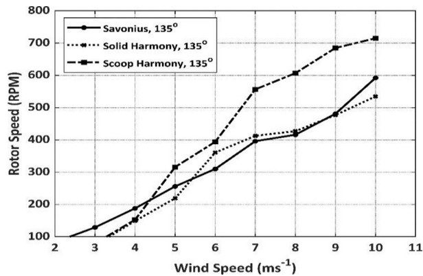
Fig. 7. Rotor Speed (RPM) performance against Wind Speed ( \text{ms}^{-1} ) for 135^\circ blade
