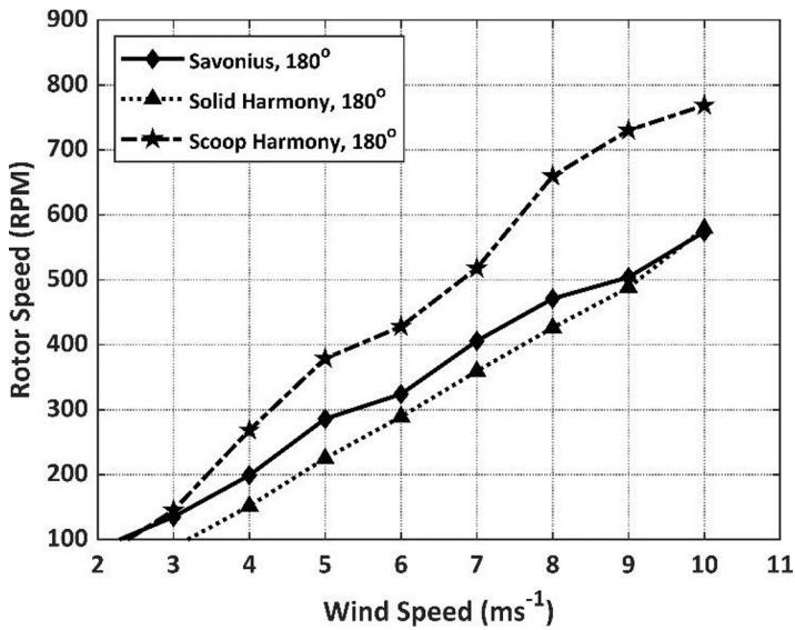
Fig. 8. Rotor Speed (RPM) performance against Wind Speed (ms -1 ) for 180° blade
