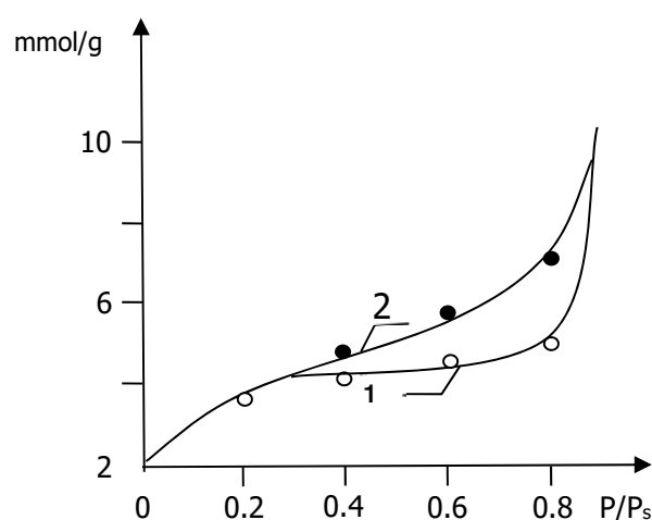
Fig. 1. Isotherm of water vapor adsorption and desorption in the dried part of the Aral Sea mobile soils.
