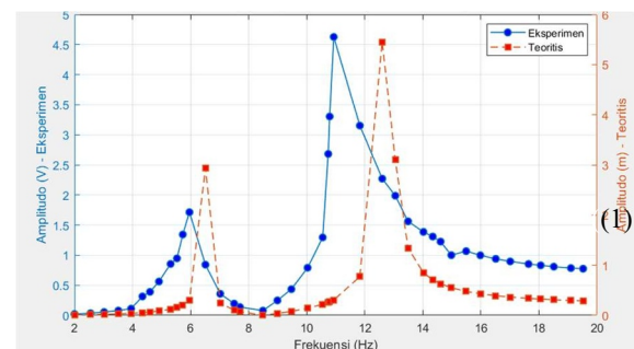
Fig. 6. Comparison graph of the experimental amplitude of two mass absorber absorber.
