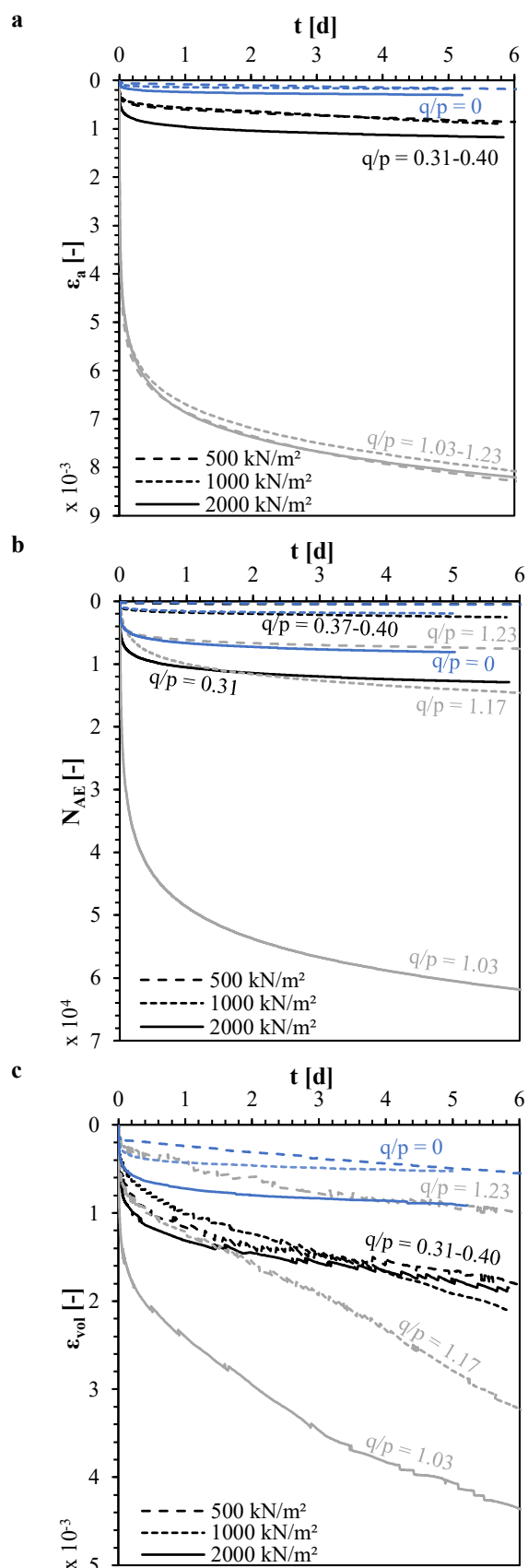
Figure 4. a Axial strain \epsilon_a , b number of AE events N_{AE} and c volumetric strain \epsilon_{vol} with time t since start of the creep phases at varying p_0 and q/p -ratios.
