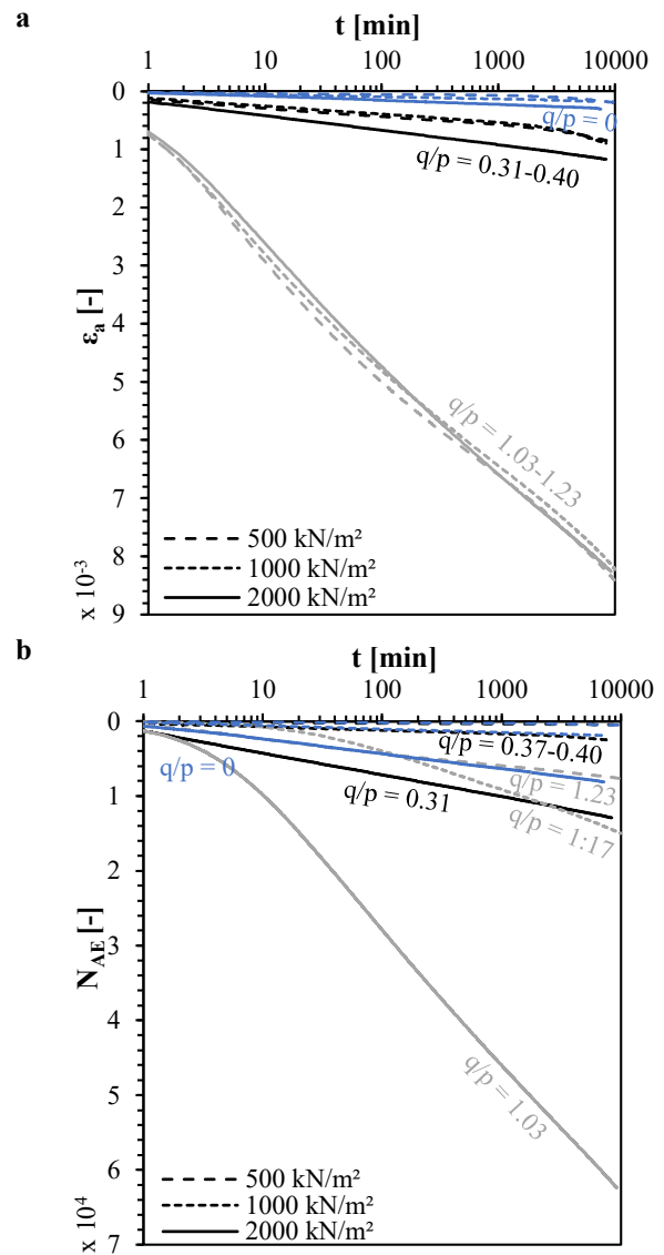
Figure 5. a Axial strain \varepsilon_a , b number of AE events N_{AE} with \log(t) for creep phases at varying p_0 and q/p -ratios.
