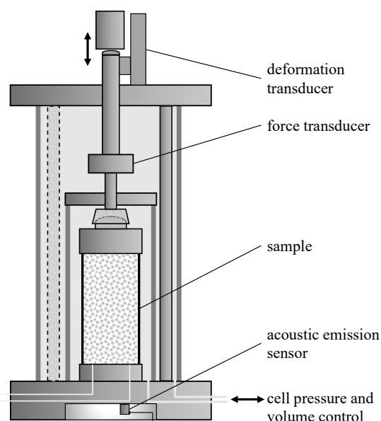
Figure 2. Schematic sketch of the used type of triaxial cell.
