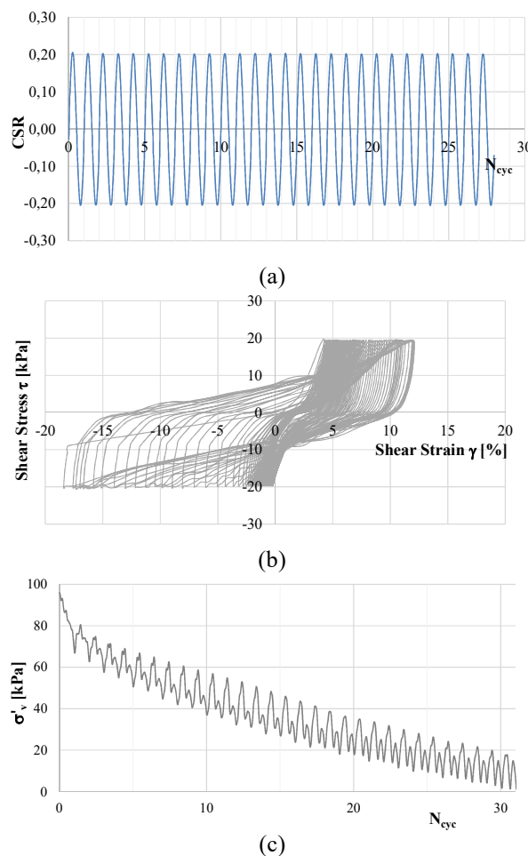
Figure 8. Results of the CSS test.
