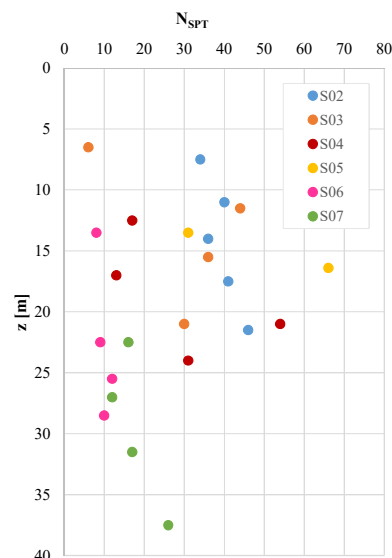
Figure 2. Results of SPT tests.
