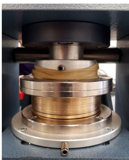
Figure 7. Restrained sample by slip rings.
