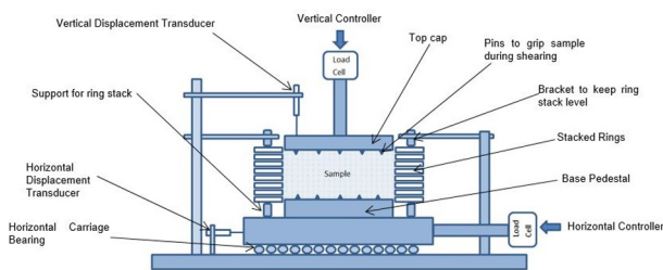
Figure 6. Scheme of the CSS apparatus.
