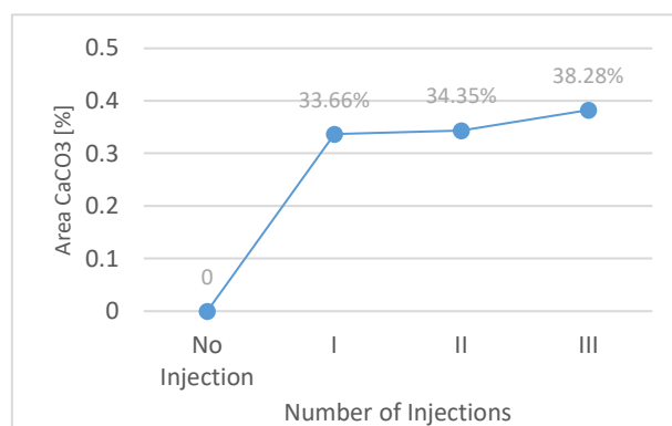
Figure 11. Amount of calcium carbonate formed as a function of the number of injections.
