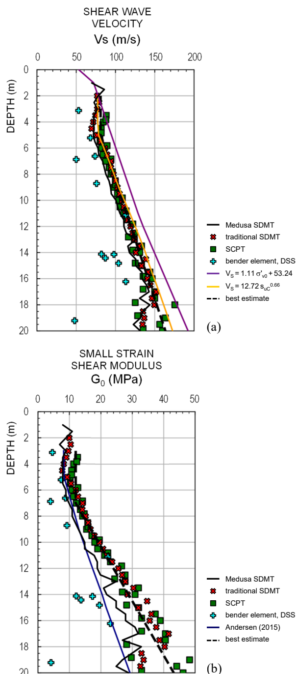
Figure 9. Comparison of profiles of V_s (a) and G_0 (b) obtained from Medusa SDMT, traditional SDMT and other tests (modified from Gundersen et al. 2019)
