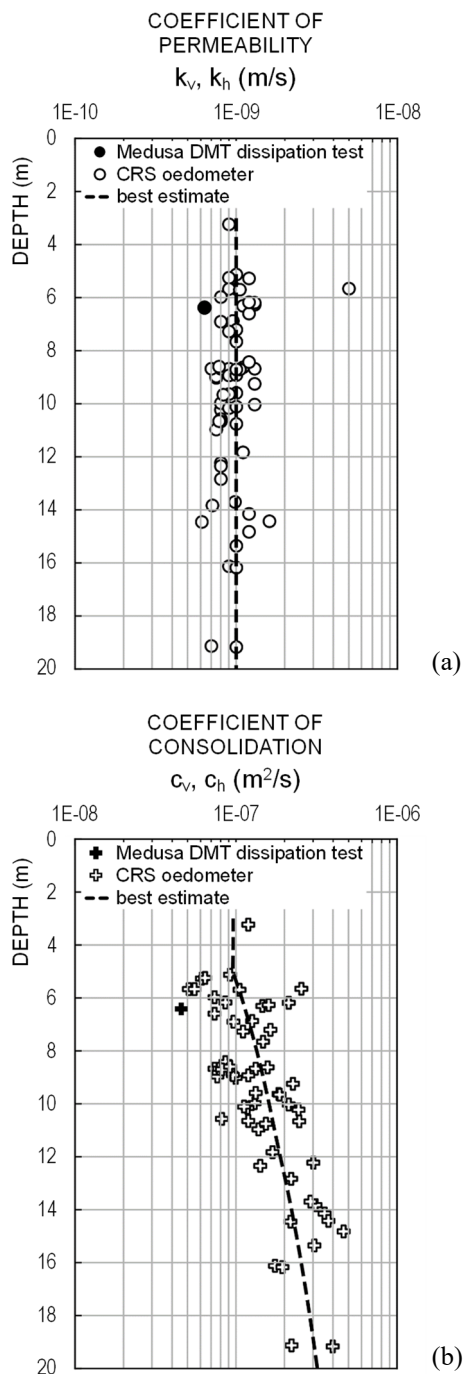
Figure 10. Comparison of coefficients of permeability (a) and consolidation (b) estimated from the Medusa DMT dissipation test ( k_h, c_h ) and obtained from laboratory CRS oedometer tests ( k_v, c_v ) (modified from Gundersen et al. 2019)
