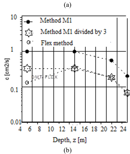
Figure 10. Szeged (a) u_2 , comparing the results of Methods I, II and III. (b) DMTA, Comparing the result of M1 in plastic soil, there is about a factor 3 difference.
