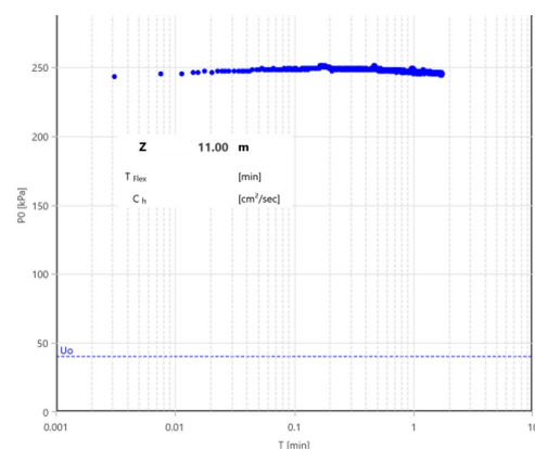
Figure 7. DMTA dissipation curve at Szeged, sand.
