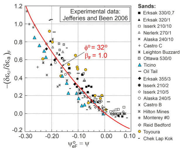
Figure 10. The relationship (\delta\epsilon_v/\delta\epsilon_a)_F - \psi_{eF}^o for sands (adapted from Prearo 2015)
