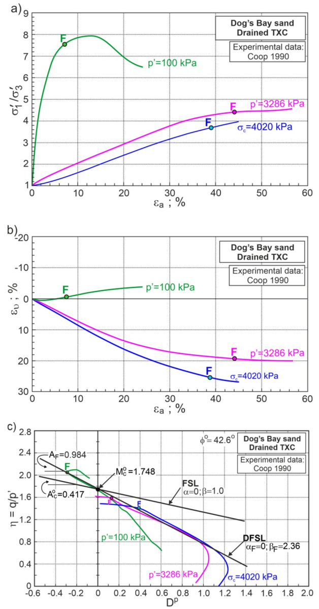
Figure 3. The relations for drained triaxial compression of Dog's Bay sand: (a) (\sigma'_1/\sigma'_3) - \alpha_a ; (b) \epsilon_v - \epsilon_a ; (c) \eta - D^p (experimental data from Coop 1990).
