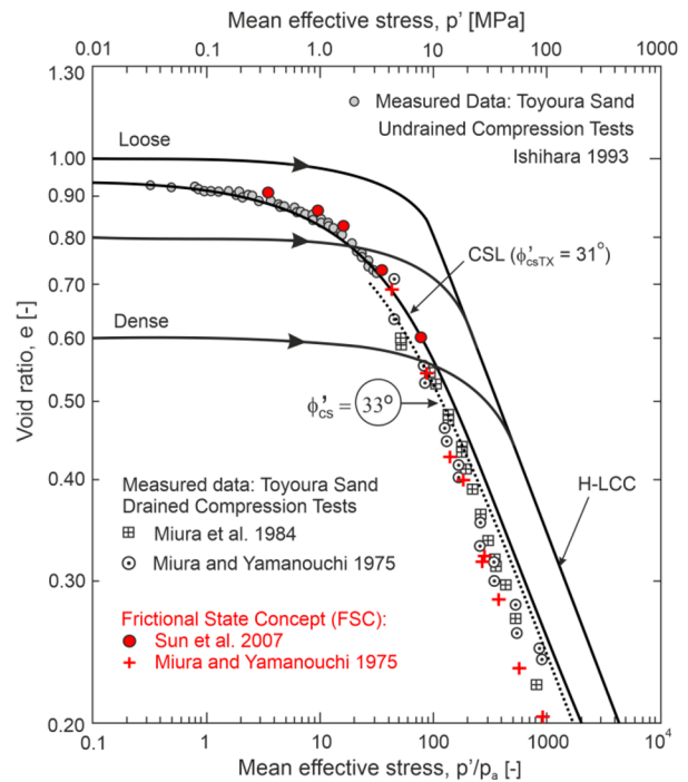
Figure 6. Critical state and critical frictional state for Toyoura sand (adapted from Pestana et al. 2002).
