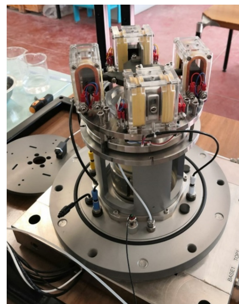
Figure 2. Resonant column / Torsional shear apparatus available at the Geotechnical Laboratory of the University of L'Aquila: compressed air cell (a) and pedestal, specimen, and driving system (b).
