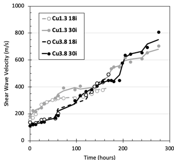
Figure 2. V_s of column specimen during MICP treatment. The trendline represents the three-point moving average. Note: 18i or 30i implies the specimen received either 18 or 30 MICP cementation injections, respectively.
