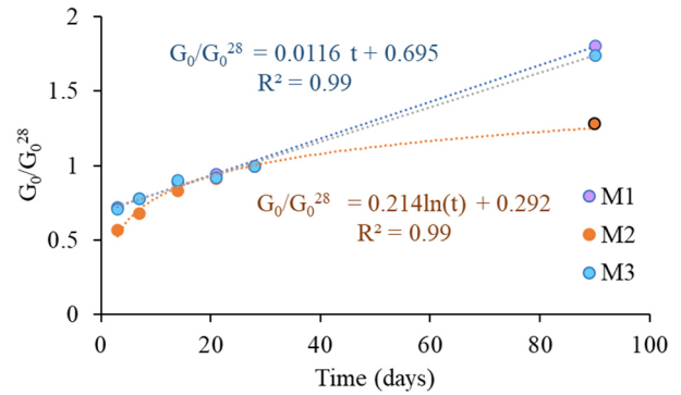
Figure 4. Stiffness evolution after 28 days.
