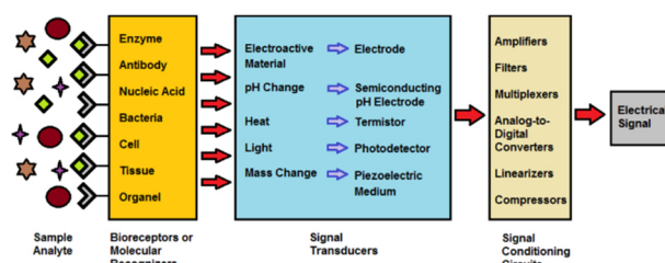
Figure 1. Biosensor operating principle: main subsystems (Vargas-Bernal et al. 2012).
