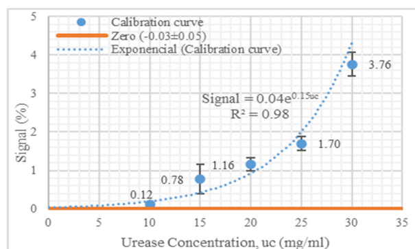
Figure 3. Calibration curve of the sensor using the magnetoresistive platform.
