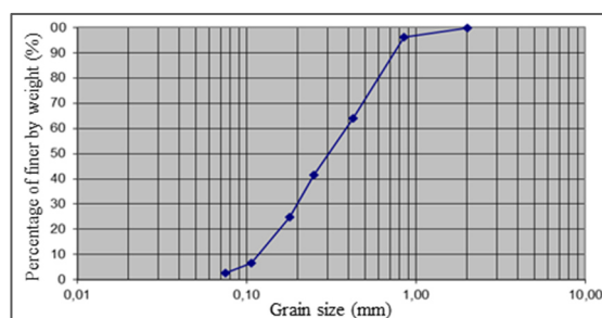
Figure 4. Grading size distribution curve of the sand.
