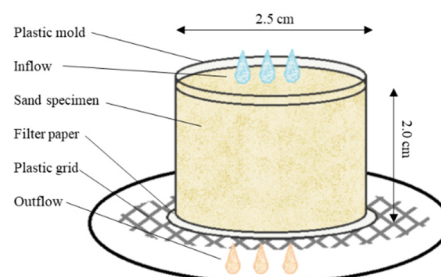
Figure 5. Setup to prepare biocemented treated soil samples.
