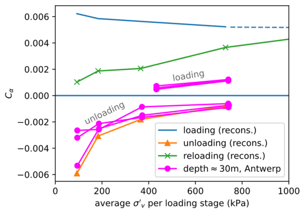
Figure 13. Secondary compression and swelling index of undisturbed Boom clay out of oedometer tests.
