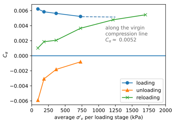
Figure 9. Secondary compression and swelling index of reconstituted Boom clay out of oedometer test.
