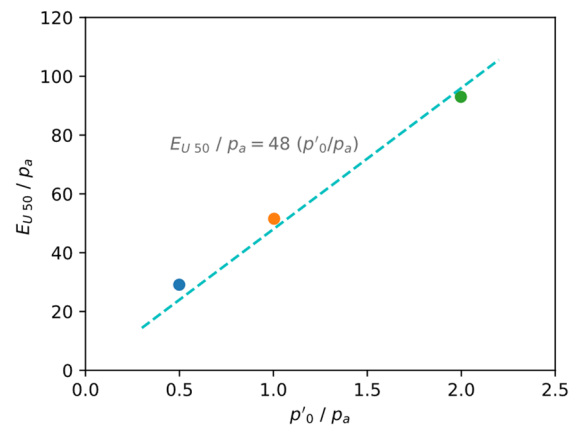
Figure 5. Undrained modulus E_{u50} vs. p'_0 normalized by the atmospheric pressure p_a = 100 kPa.
