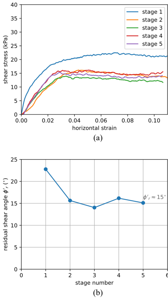
Figure 6. Residual strength of reconstituted Boom clay under a normal effective stress of 50 kPa.
