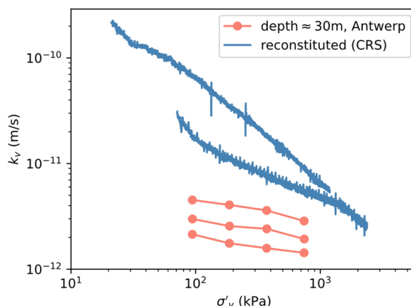
Figure 12. Vertical hydraulic conductivity of undisturbed Boom clay out of oedometer tests.
