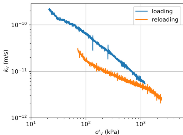
Figure 8. Evaluation of the vertical hydraulic conductivity of reconstituted Boom clay out of CRS test.
