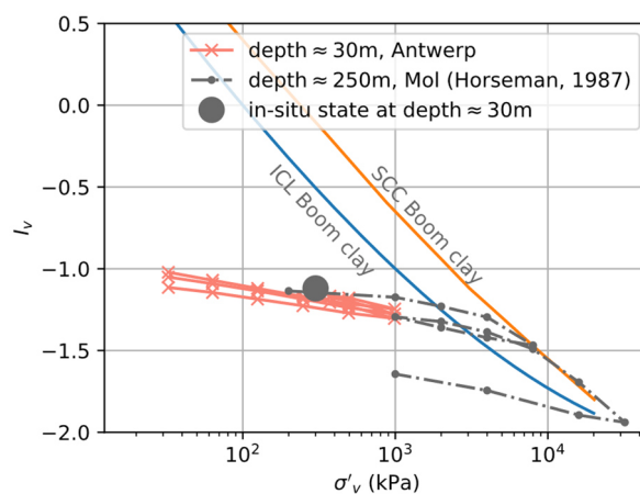
Figure 11. Normalized compression curves of undisturbed Boom clay samples.
