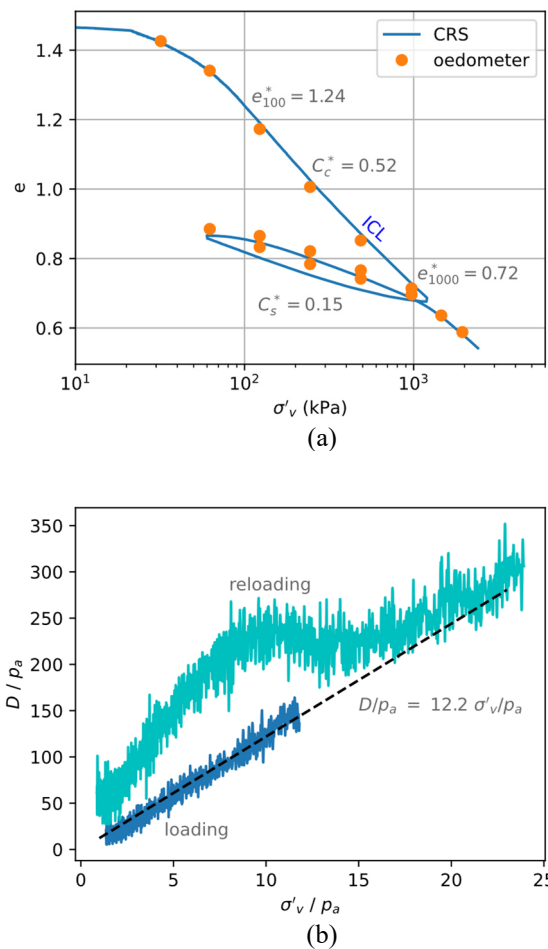
Figure 7. 1D compression of reconstituted Boom clay (a) out of CRS and oedometer (b) constrained modulus D .
