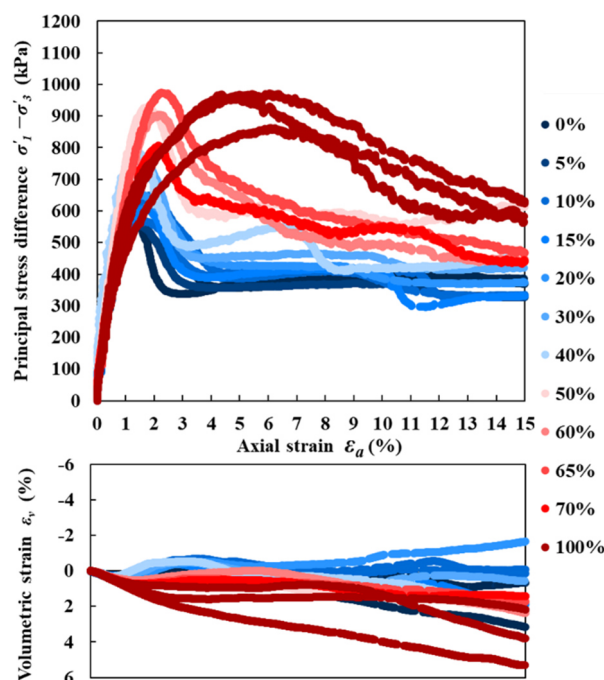
Figure 5. Stress-strain relationship
