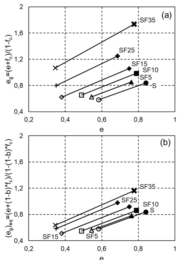
Figure 3. Variation of void ratio, e , with a) intergranular void ratio, e_g , and b) equivalent intergranular void ratio, (e_g)_{eq} , for the tested sand-silt mixtures up to the threshold fines content, f_{cth} = 35\% , based on their e_{max} and e_{min} values.
