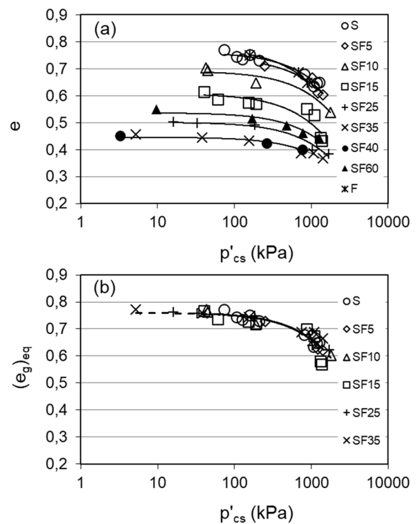
Figure 2. Critical State Lines of the sand-silt mixtures on the (a) e-p'_{cs} and (b) (e_g)_{eq}-p'_{cs} plane.
