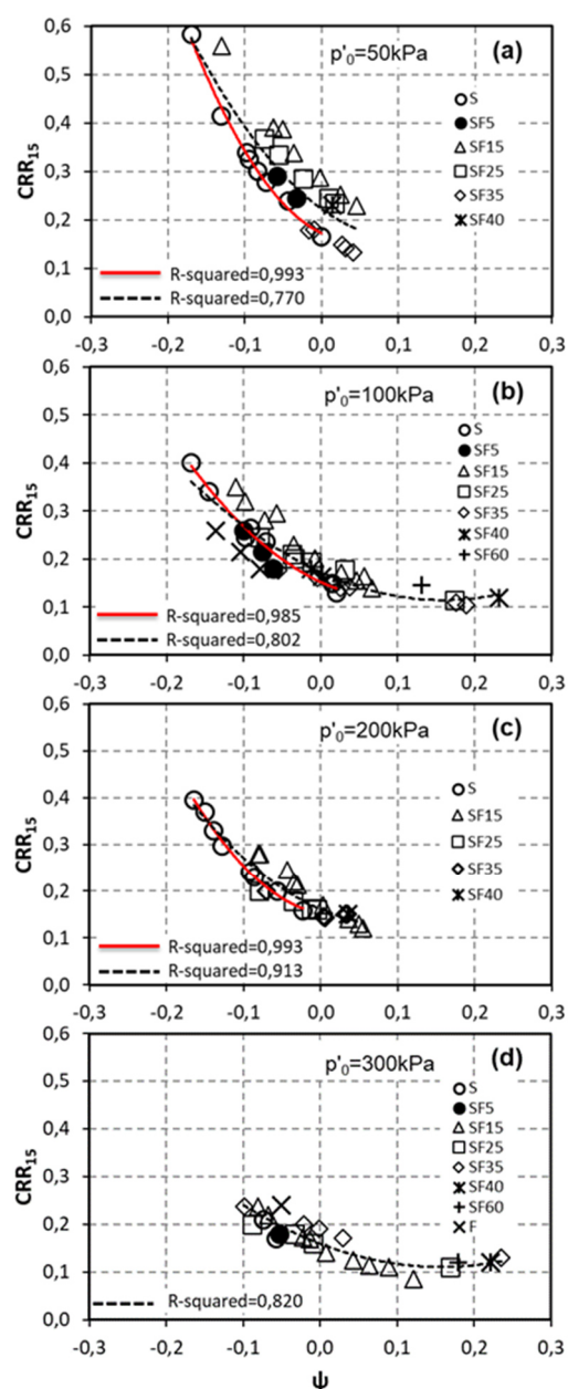
Figure 10. Variation of CRR_{15} with \psi , for the tested sand-silt mixtures, at the effective stresses, p'_0 , of (a) 50\text{kPa} , (b) 100\text{kPa} , (c) 200\text{kPa} and (d) 300\text{kPa} .
