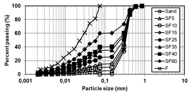
Figure 1. Grain size distributions of the tested materials.
