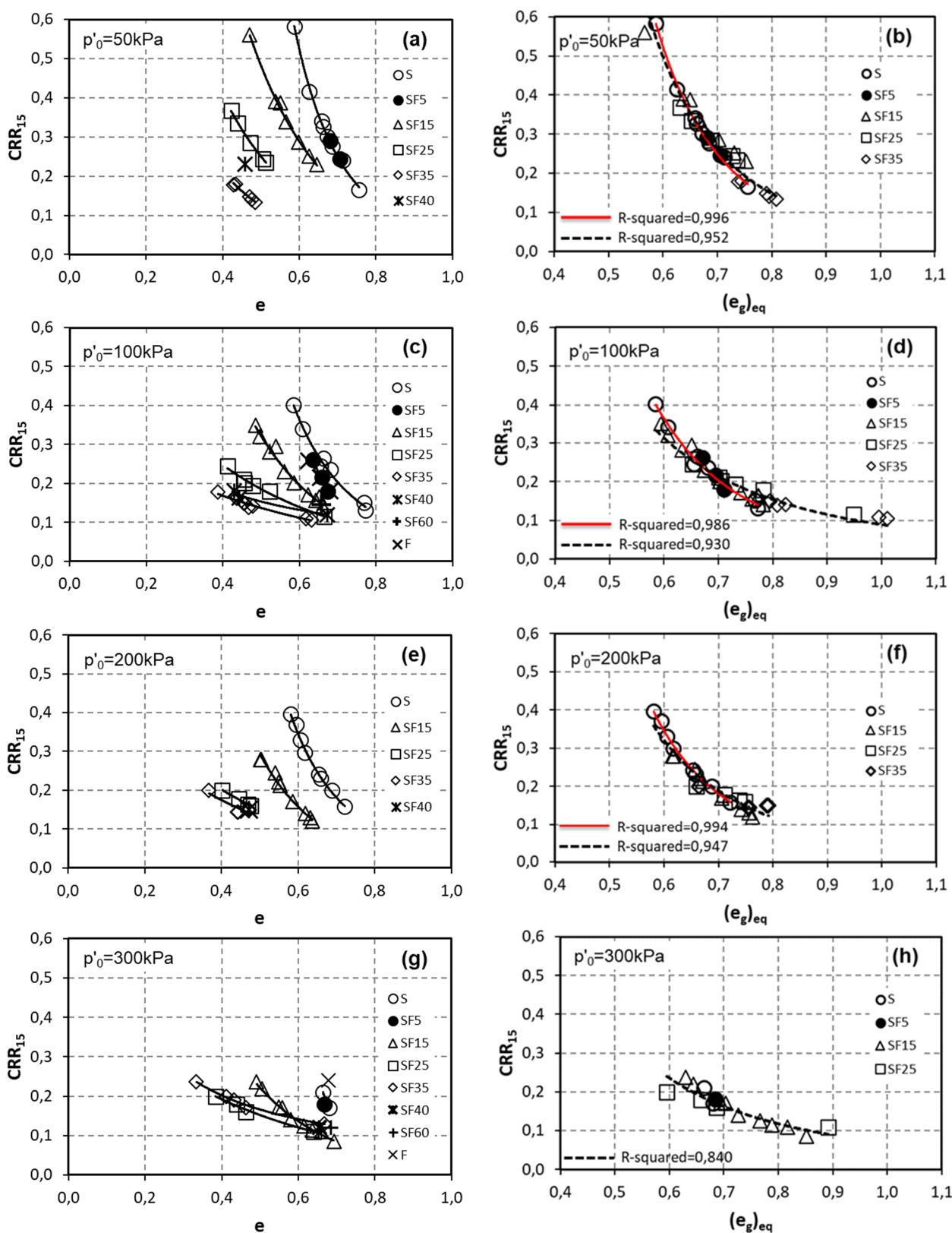
Figure 8. Liquefaction Resistance curves of the sand-silt mixtures on the (a, c, e, g) CRR_{15} - e and (b, d, f, h) CRR_{15} - (e_g)_{eq} plane, at the effective stresses of p'_0=50, 100, 200 and 300 kPa.
