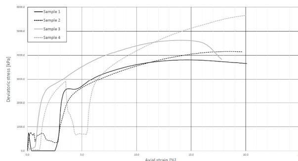
Figure 5. Deviatoric curves, test 1 at -5°C
