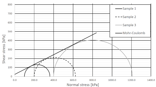
Figure 17. Test 3 at a temperature of 5°C
