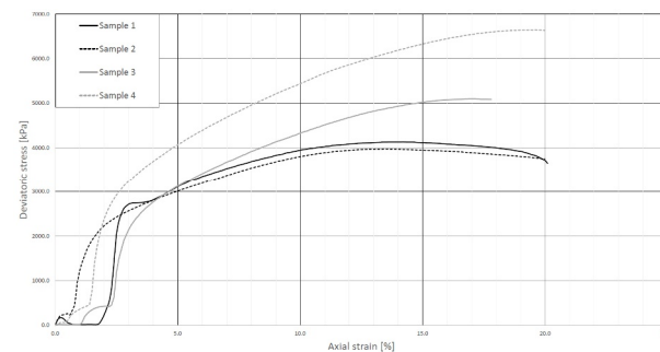
Figure 6. Deviatoric curves, test 2 at -5°C
