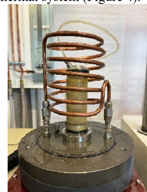
Figure 4. System assembly
