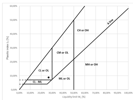
Figure 2. USCS classification
