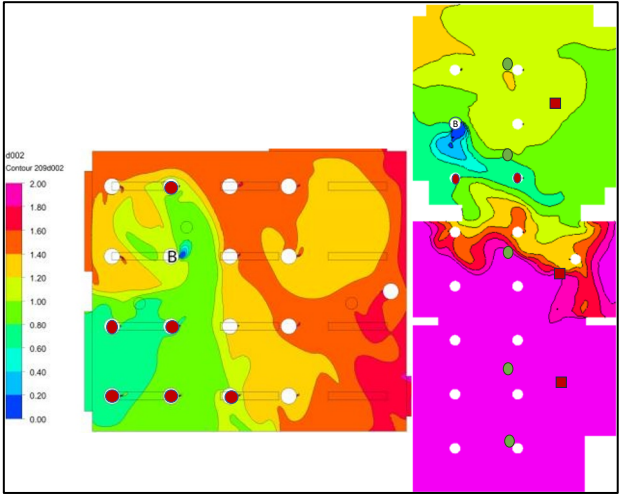
Fig. 7. Local air quality in case of infector B Left: Small classroom Right: Larger Classroom
