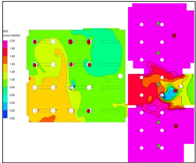
Fig. 8. Local air quality in case of infector C Left: Small classroom Right: Larger Classroom
