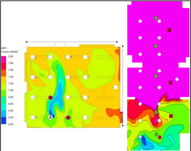
Fig. 6. Local air quality in case of infector A Left: Small classroom Right: Larger Classroom
