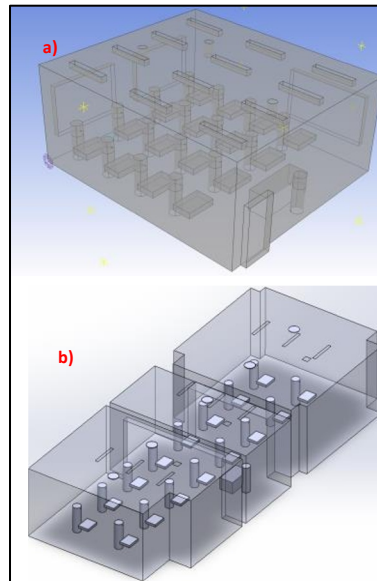
Fig. 2. CFD domain of classroom space a) Smaller classroom b) Larger classroom
