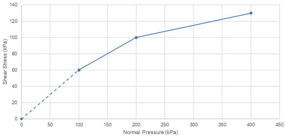
Fig. 6. Shear interface function between GCL and residual soil.
