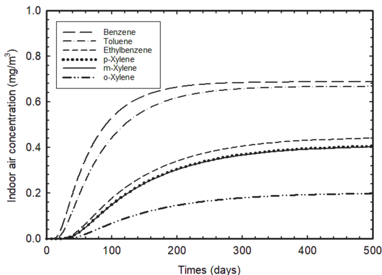
Fig. 1. Change in BTEX concentration in indoor air with time at the interface between the concrete floor and the building air in a simulated warehouse with a 4.1 mm BGM installed as a vapour barrier.
