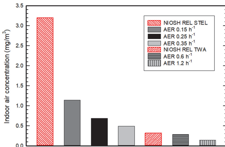
Fig 2. Peak indoor air concentration for benzene at the interface between the concrete floor and the building air for different air exchange rates in a simulated warehouse with a 4.1 mm BGM installed as a vapour barrier.
