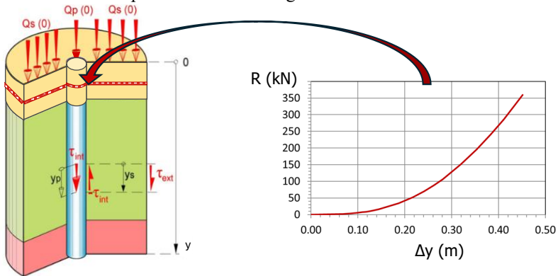
Figure 3. Relationship between the geosynthetic displacement \Delta y and the load R
