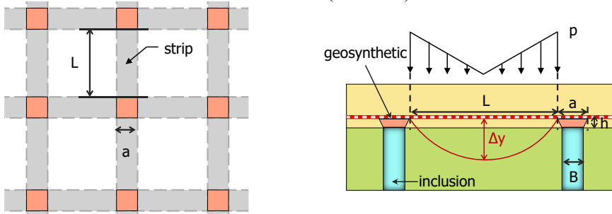
Figure 4. Triangularly distributed load
