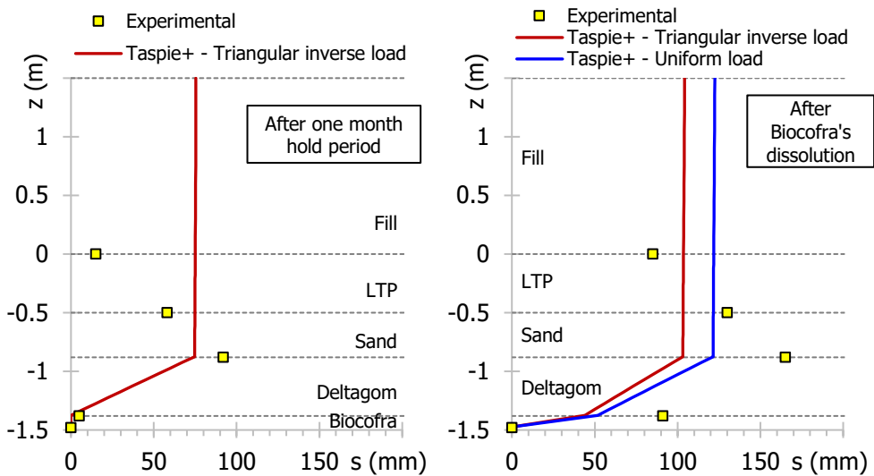
Figure 9. Vertical displacements - with geosynthetic - Test plot 5 - Phase 3 and Phase 5
