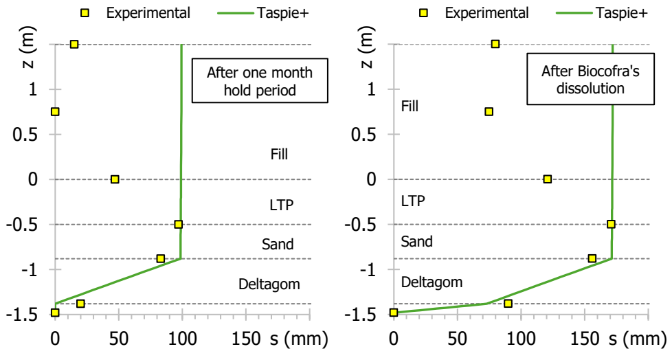
Figure 8. Vertical displacements - without geosynthetics - Test plot 1 - Phase 3 and Phase 5
