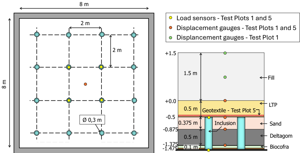
Figure 7. Geometry - Full-Scale Tests CEREMA Rouen – Test Plot 1 and Test Plot 5 [5]
